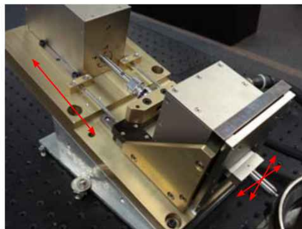
Multi-Axis LXY15 and LAL95
